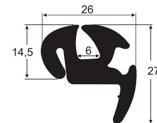
8030 SBR 60 Sh A Vigia Central Scania
