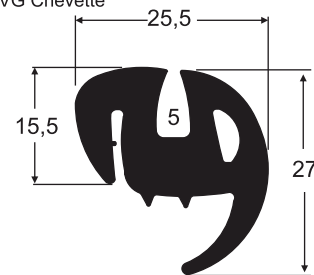
8008 SBR 60 Sh A PB/VG Chevette
