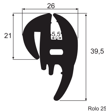
8020 SBR 70 Sh A Parabrisa Mercedes Ben Cabine Alta 75/89
