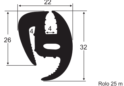
8020 SBR 70 Sh A Parabrisa Mercedes Ben Cabine Alta 75/89
