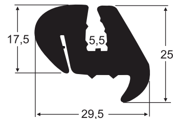
8008 SBR 60 Sh A PB/VG Chevette
